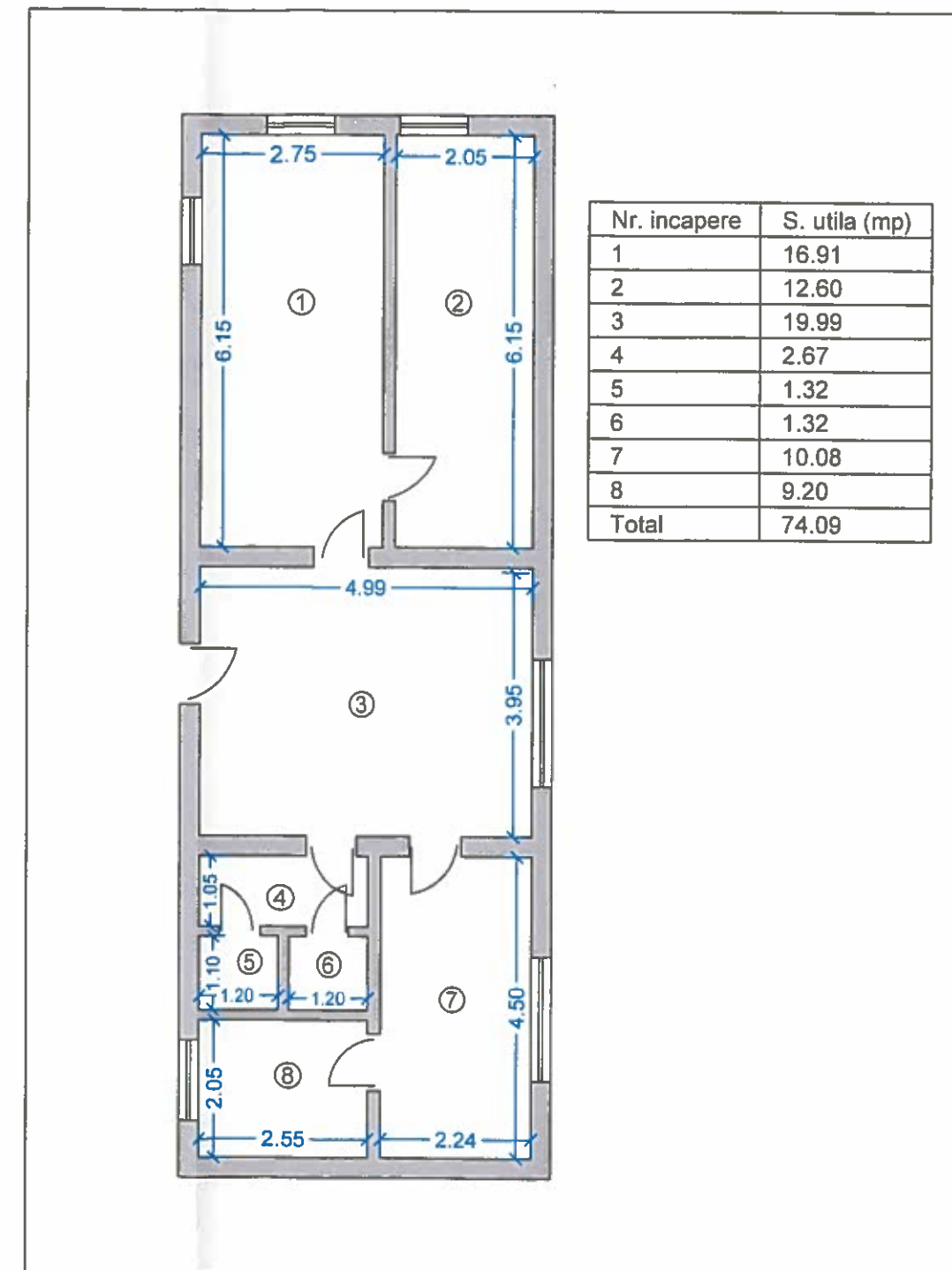
Relevu C1 Scara 1:100
